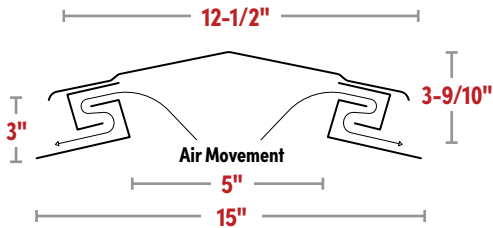
Roofline IV – 221 Sq. In. Free Air Space Manufactured to a 4:12 pitch; adjusts from 2:12 to 8:12
