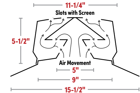
Roofline II – 400 Sq. In. Free Air Space Manufactured to a 4:12 pitch; adjusts from 2:12 to 5:12
